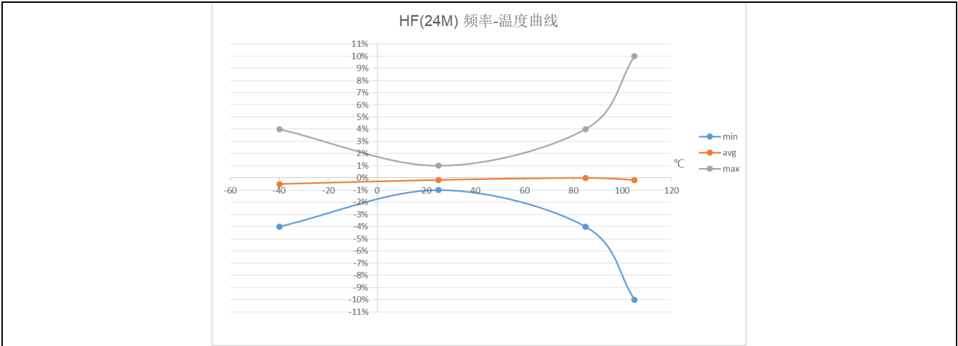
Figure 3-10 HF(24M)频率温度曲线
